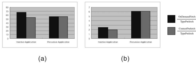
Fig. 11. Experimental results for iterative-application and recursive application. (a) Relative number of fetches and (b) relative elapsed time.
